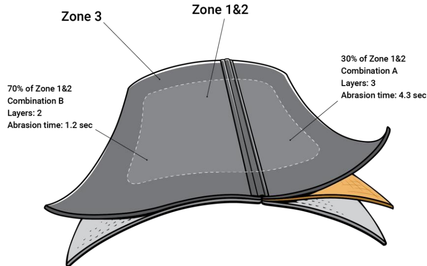
Figure 3.3 Illustration of two fabric combinations within the one Zone area.
