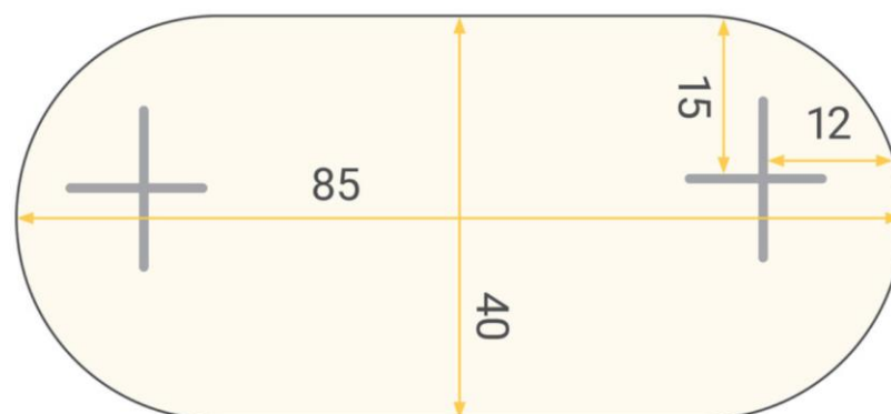
Figure 5.5 Template for assessing size of knuckle impact protector (dimensions in mm)
