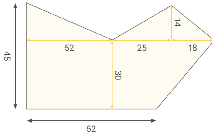
Figure 5.6 Template for assessing size of palm impact protector (dimensions in mm)
