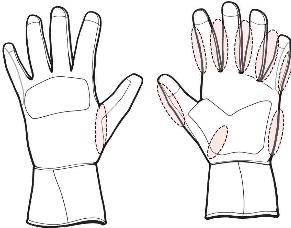
Figure 5.4 Location for tensile seam strength samples from gloves
