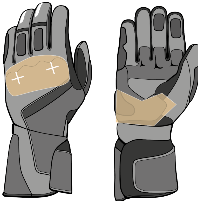
Figure 5.7 Placement of glove impact protector templates
